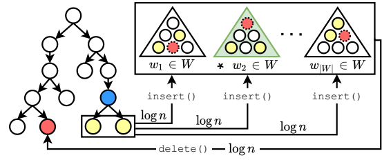
Figure 3: A modified implementation of anytime weighted A* that manages multiple open lists for different weights.
